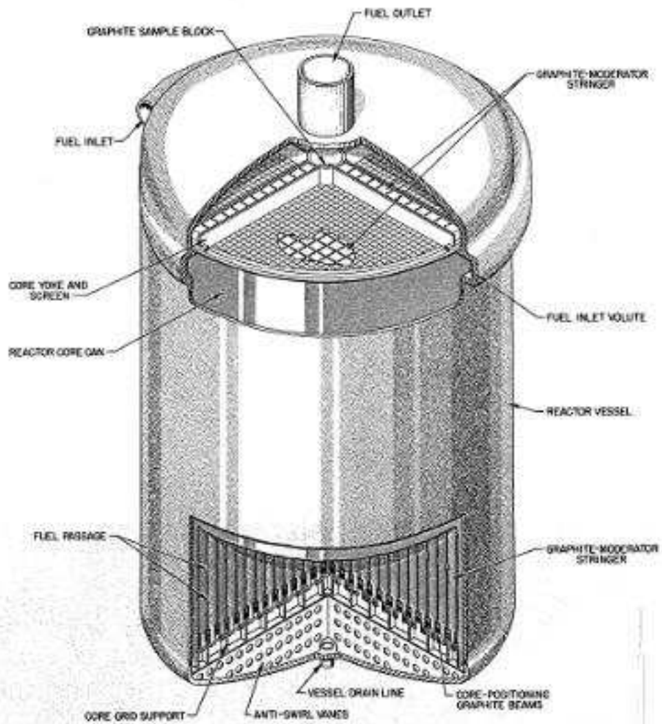
Fig. 1.2. MSRE Reactor.
