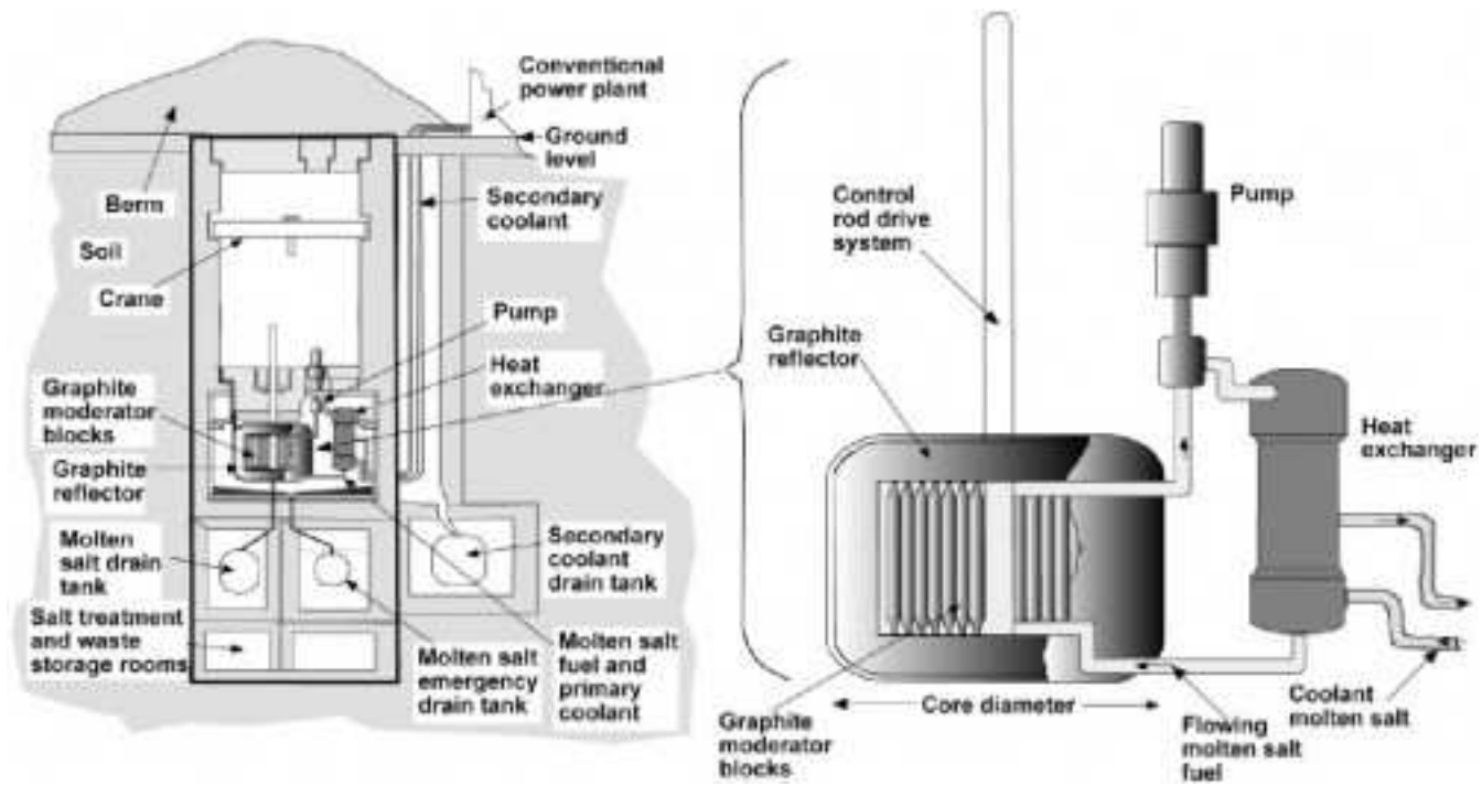
Figure 3: DMSR underground
